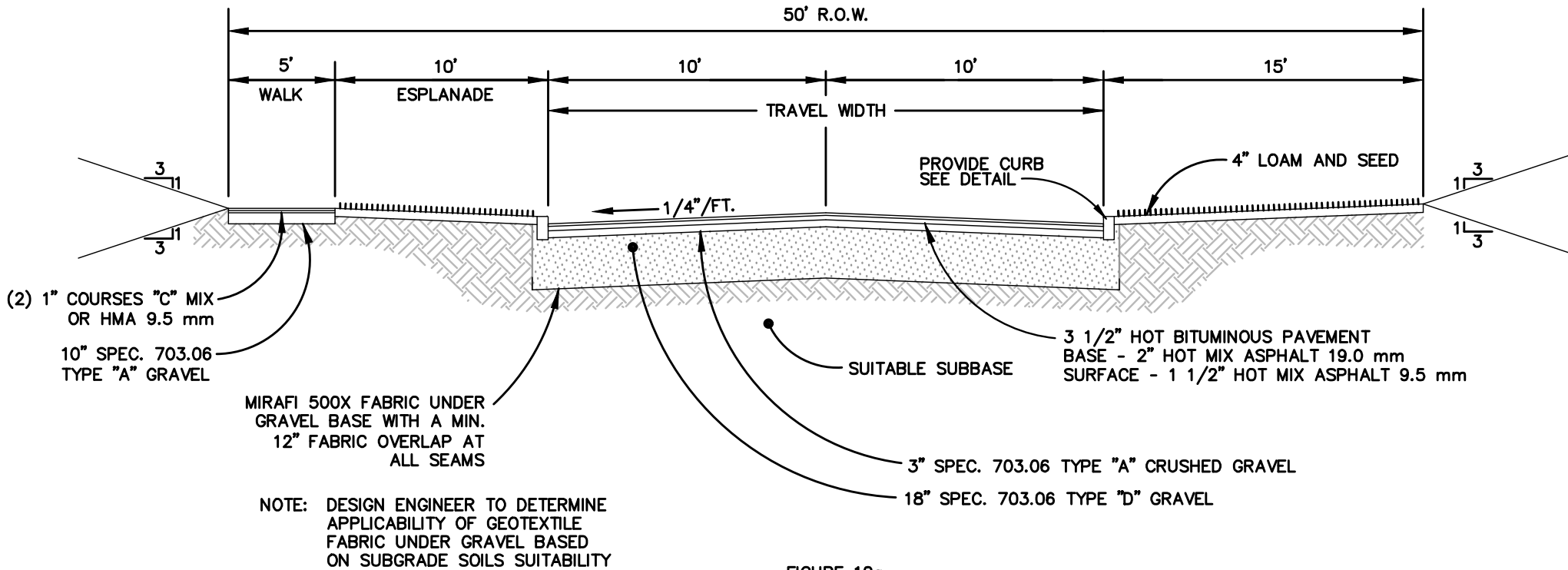
FIGURE 10a URBAN PAVED PRIVATE WAY NTS
