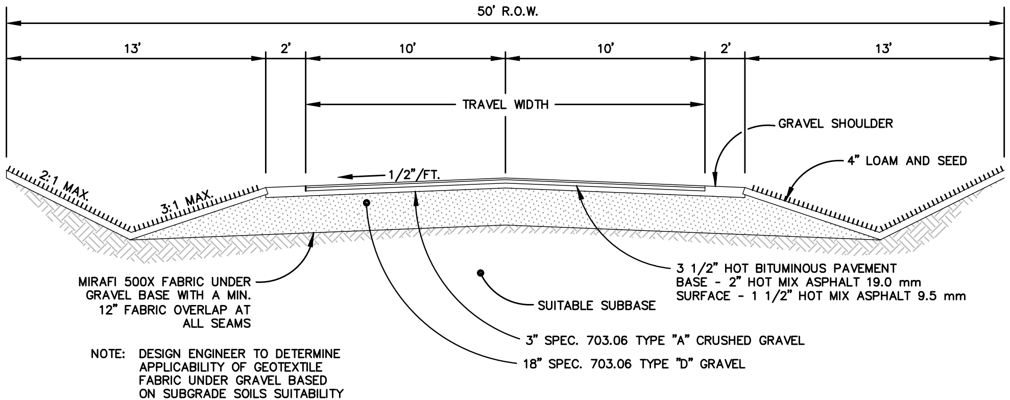
FIGURE 10b RURAL PAVED PRIVATE WAY NTS
